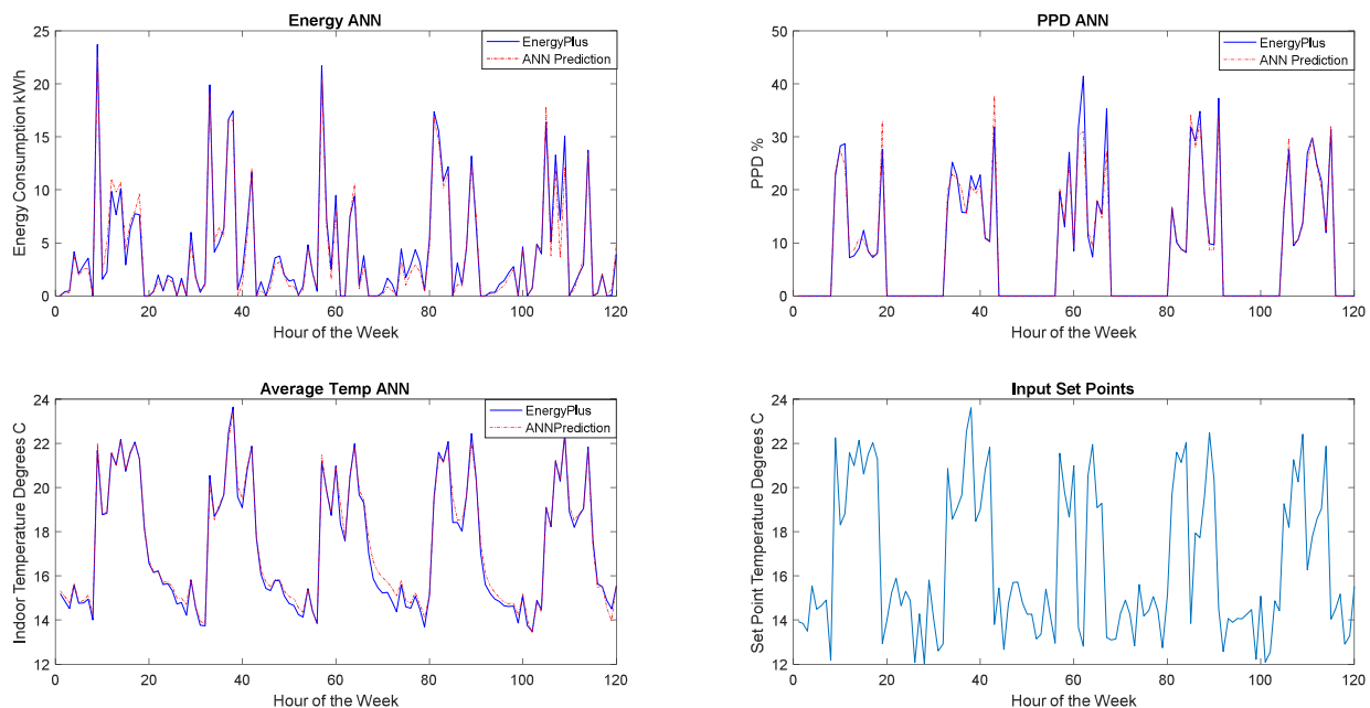
Fig. 3. ANN Prediction vs Energy Plus Prediction
