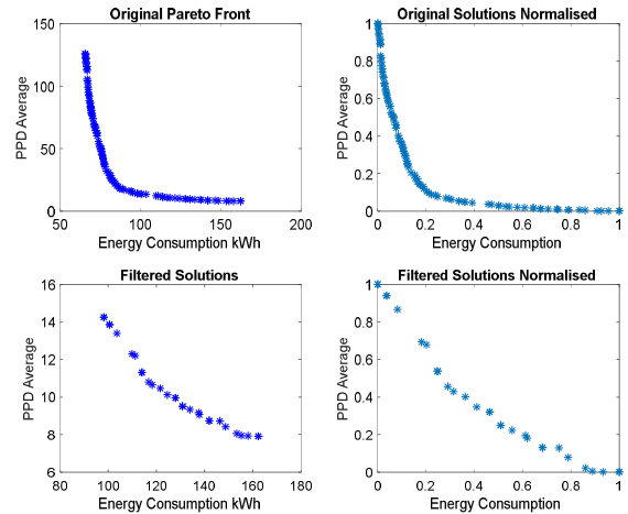
Fig. 5. Solution Filtering Example
