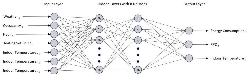
Fig. 2. ANN Inputs and Outputs
